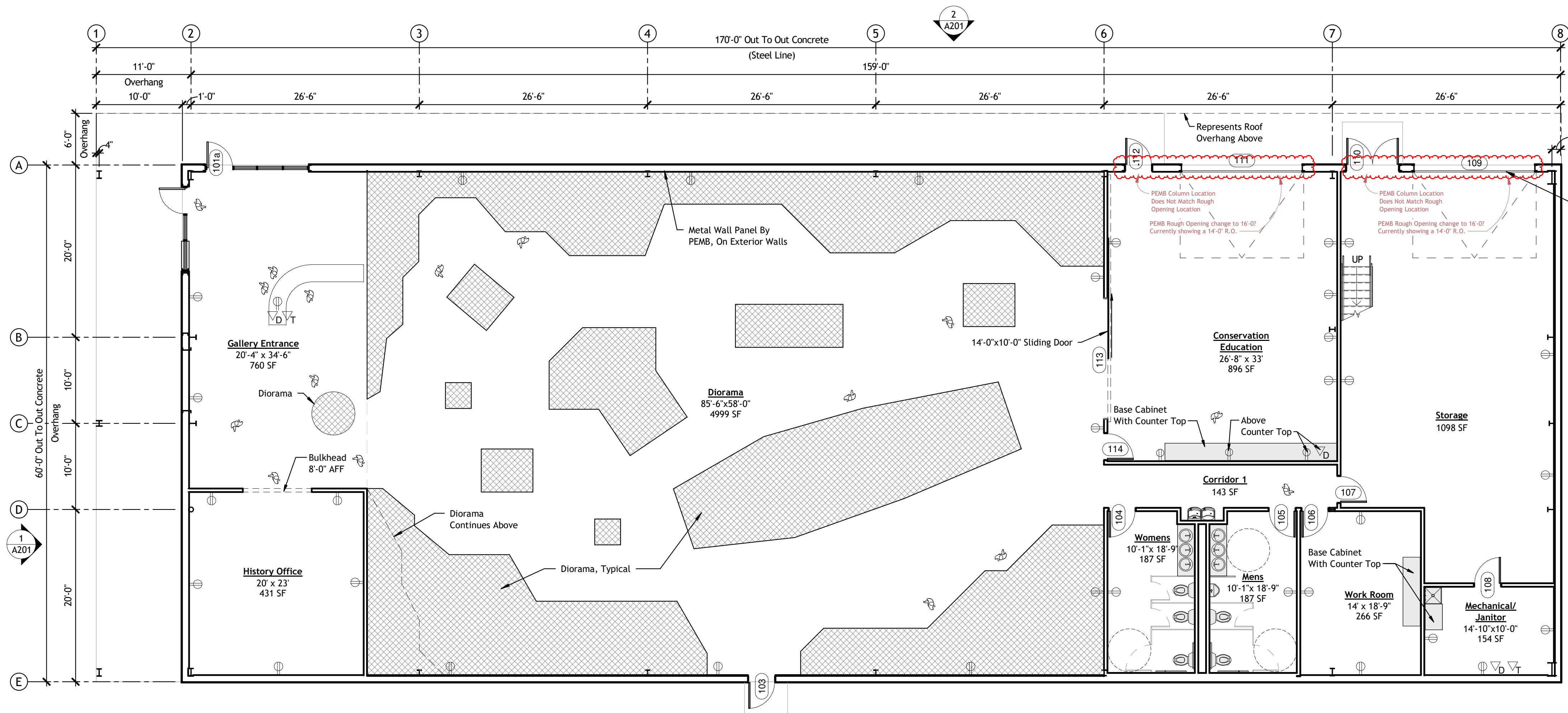
Floor Plan SCALE: 1/8" = 1'-0" Sketch 01 - 03/21/24
