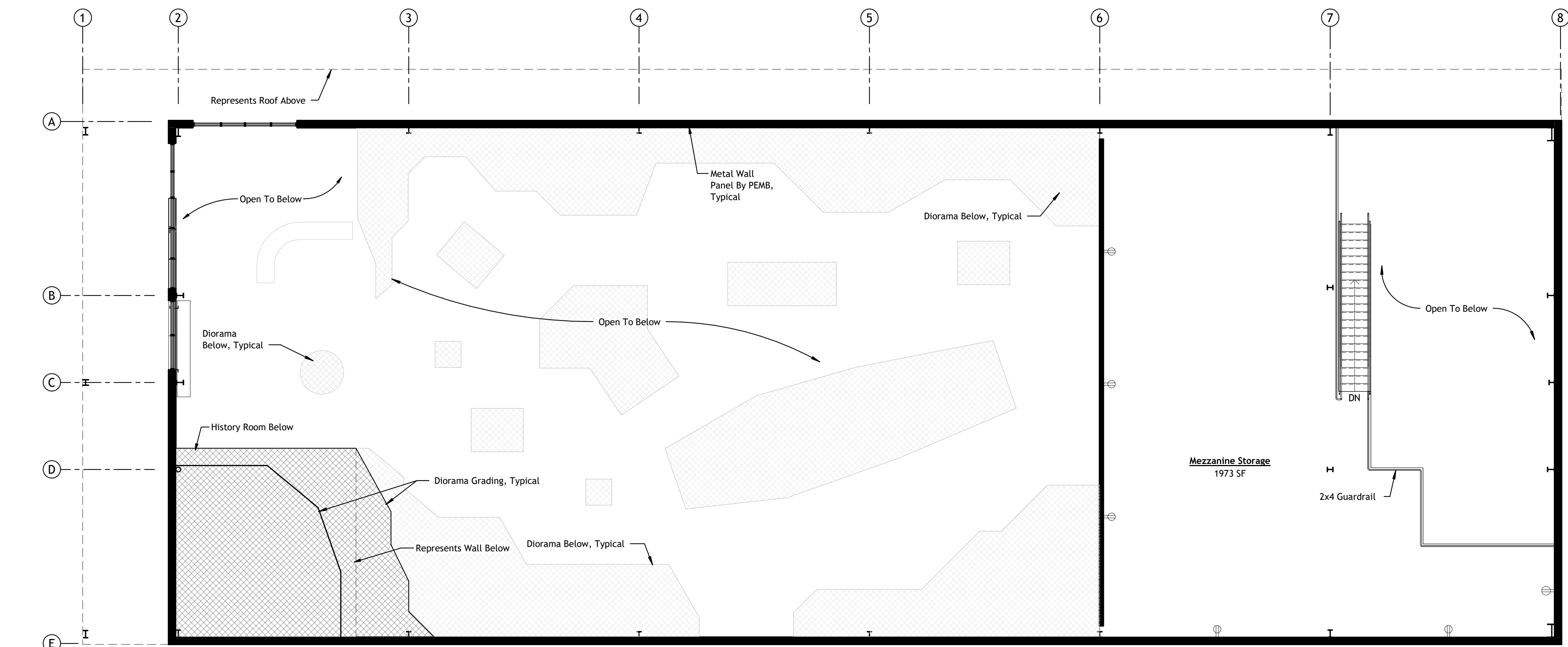
Mezzanine Plan SCALE: 1/8" = 1'-0" Sketch 01 - 03/21/24
